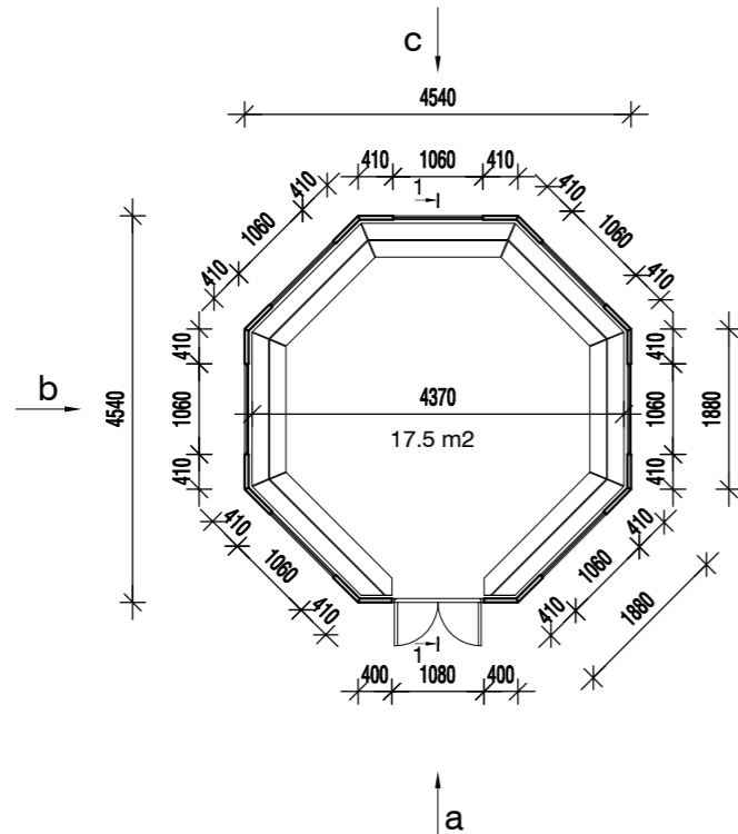
FLOOR PLAN
